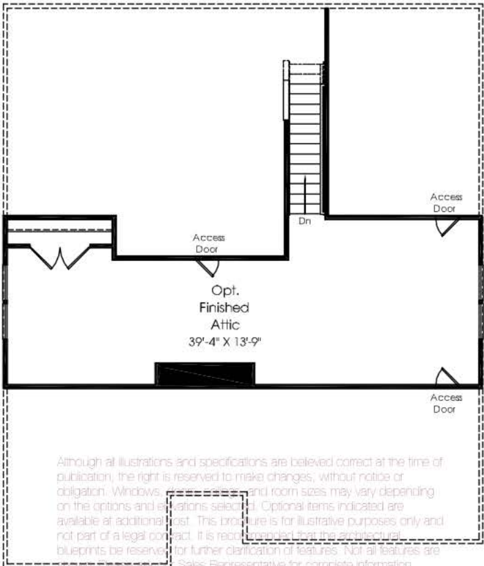
Opt. Finished Attic
