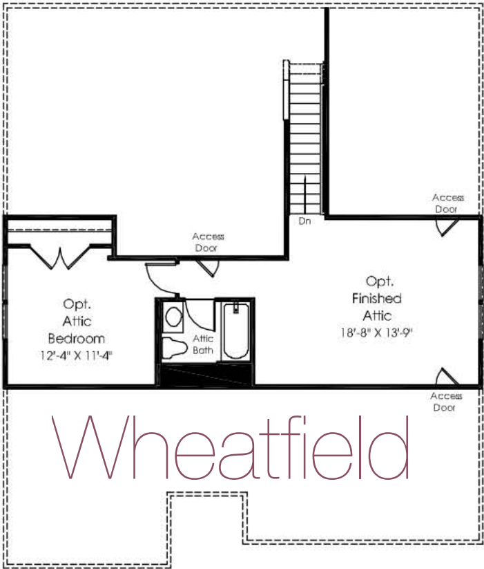
Opt. Attic Bedroom
